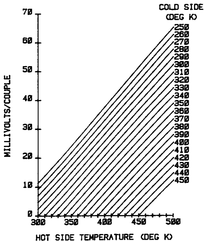
Figure 5. Voltage per couple of a thermoelectric module at maximum efficiency as a function of junction temperatures.
